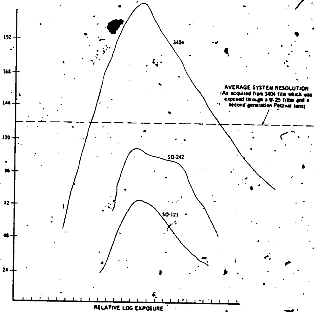
Graphic 5a. FILM/SYSTEM RESOLUTION CAPABILITY (1.7:1 Contrast Ratio)
