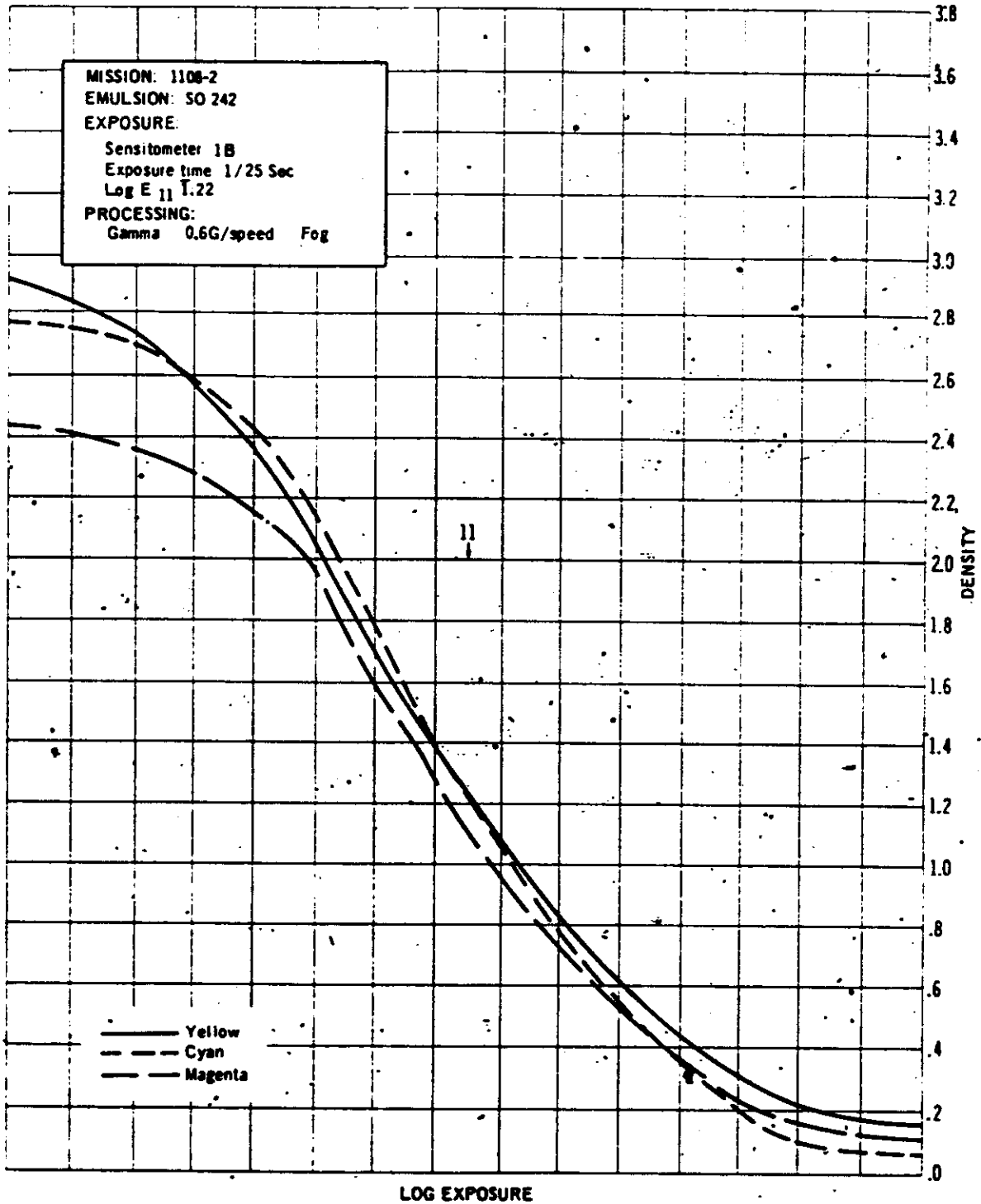
GRAPHIC 8a. PROCESS CONTROL CURVES (HEAD)
