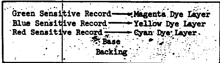
GRAPHIC 3a. CROSS SECTIONS OF SO-121 AND SO-242
