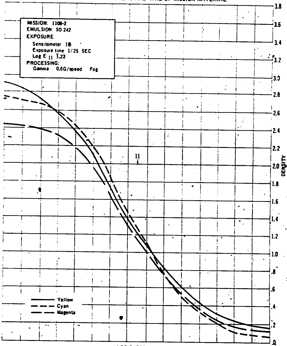
GRAPHIC 9a. PROCESS CONTROL CURVES (TAIL)
